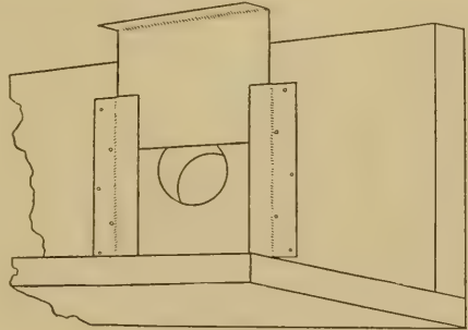
FIG. 1.—Sliding gate in flume.
